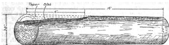
FIG. 6.—Deduction for defect caused by fire scar
