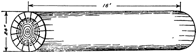
FIG. 12.—Deduction for defect caused by wind checks
